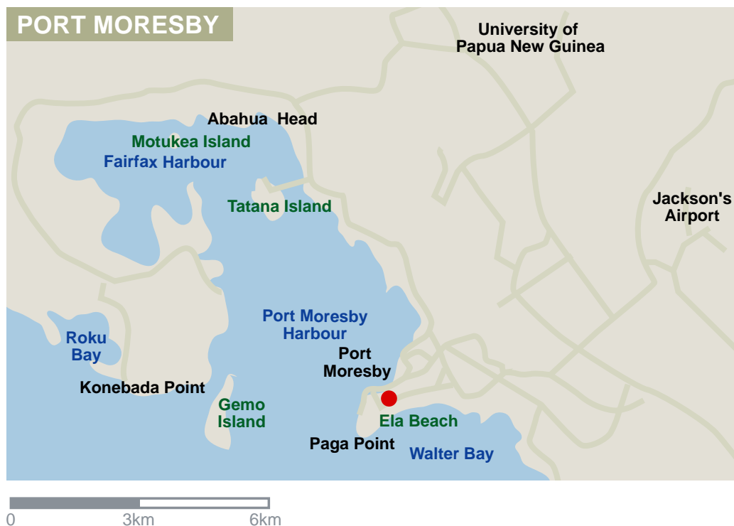
Port Moresby location map
